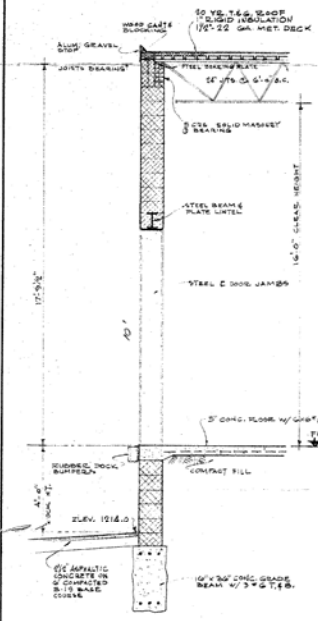
WALL SECTION 'A' SCALE 3/8"=1'
